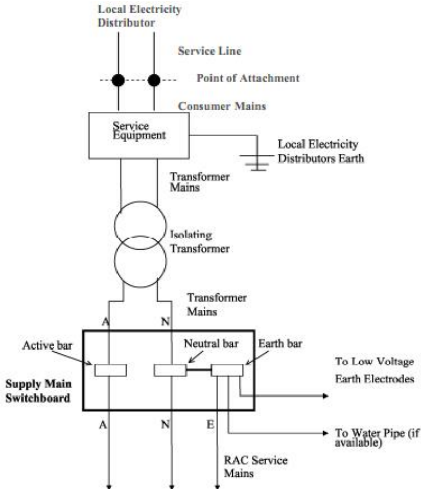
Figure 2 Supply from Local Electrical Distributors Network
