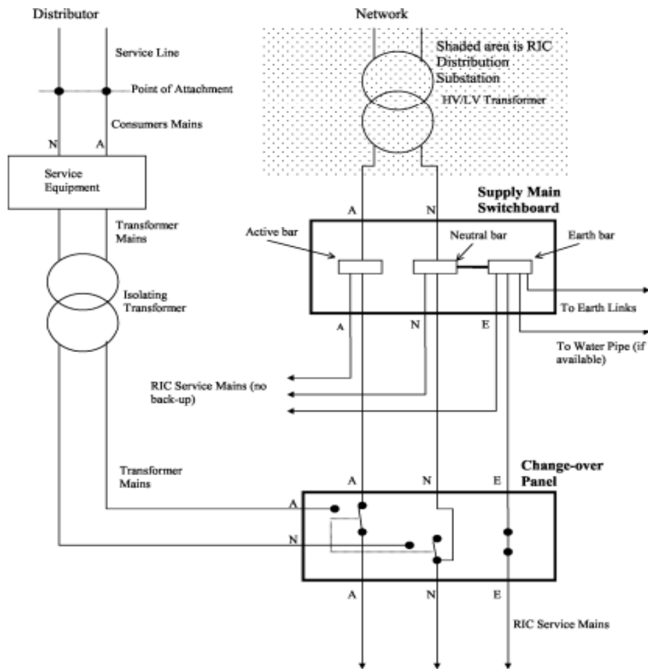
Figure 3 Back-up Supply with Change-over Contactor
